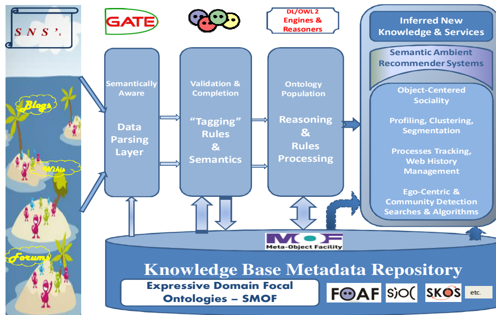
Fig 1. General overview of the proposed real-time knowledge-based architecture and modeling platform.
