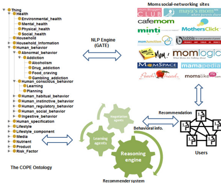
Fig. 2. COPE ontology as basis for appropriate recommendations based on inferred knowledge from users’ behaviors and activities.
