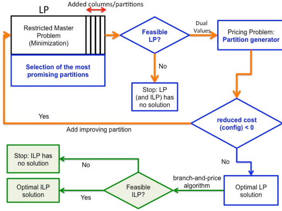
Figure 2: Overview of ILP solution process
